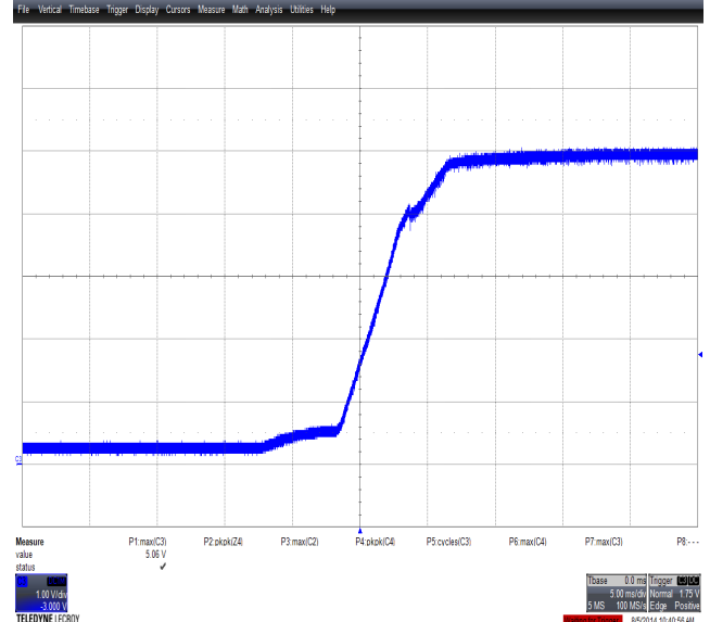
Figure 16 – 5 V Start-up Profile, Full Load; 265 VAC; 1 V / div., 5 ms / div.
