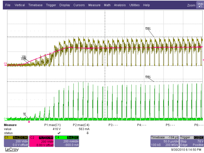
Figure 42 – 230 VAC / 50 Hz, 45° Dimming Phase Angle. 6 LED in Series (18.2 V / 350 mA) Ch1(Yellow): V_{DS} , 200 V / div. Ch2(Red): V_{IN} , 200 V / div. Ch4(Green): I_{DS} , 200 mA / div., 50 \mu s / div.
