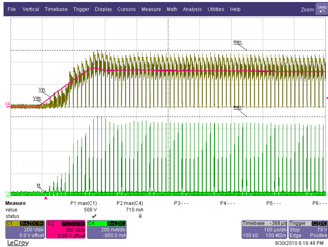
Figure 44 – 230 VAC / 50 Hz, 90° Dimming Phase Angle. 6 LED in Series (18.2 V / 350 mA) Ch1(Yellow): V_{DS} , 200 V / div. Ch2(Red): V_{IN} , 200 V / div. Ch4(Green): I_{DS} , 200 mA / div., 100 \mu s / div.
