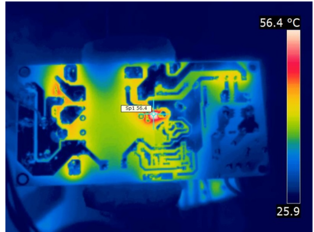
Figure 19 – Blocking Diode D4 (Sp1) Case Temperature.
