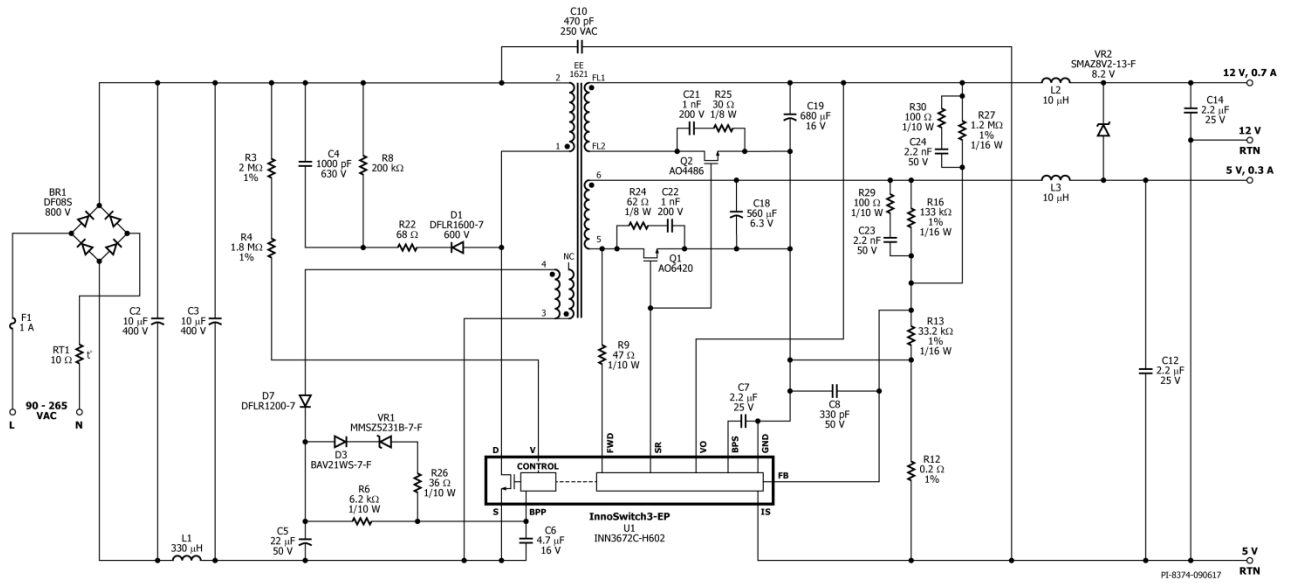
Figure 3 – Schematic.
