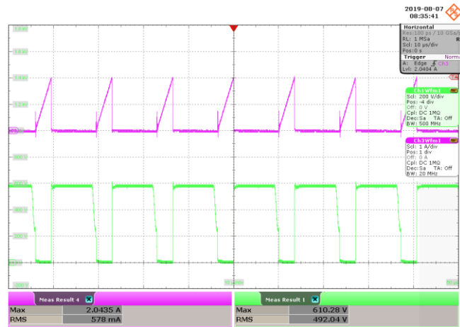
Figure 88 – 305 VAC, 48 V LED Load. Upper: I_{DRAIN} , 1 A / div. Lower: V_{DRAIN} , 200 V / div., 10 μs / div.
