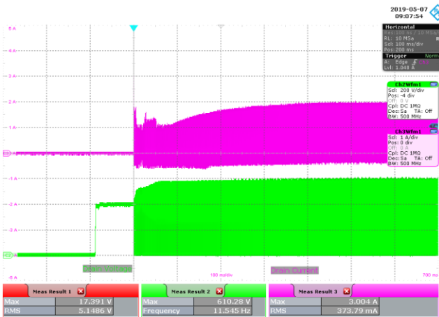
Figure 91 – 277 VAC, 48 V LED Load. Upper: I_{DRAIN} , 1 A / div. Lower: V_{DRAIN} , 200 V / div., 100 ms / div.
