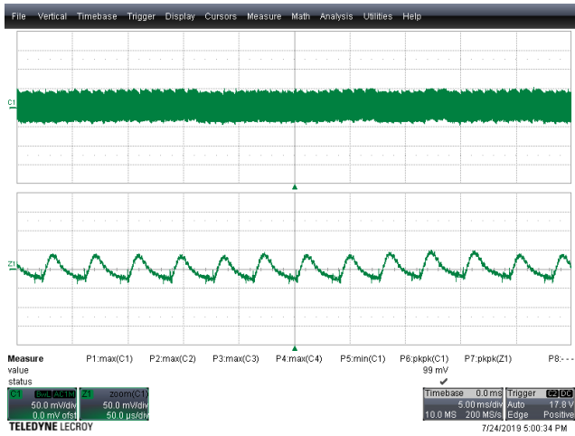
Figure 87 – Output Voltage Ripple. V_{IN} = 130 \text{ VDC} , I_{OUT} = 0.625 \text{ A} . Top Half: V_{OUT} , 50 mV, 5 ms / div. Bottom Half: Zoom @ 50 \mu\text{s} / div. V_{RIPPLE} = 99 \text{ mV}_{P-P}
