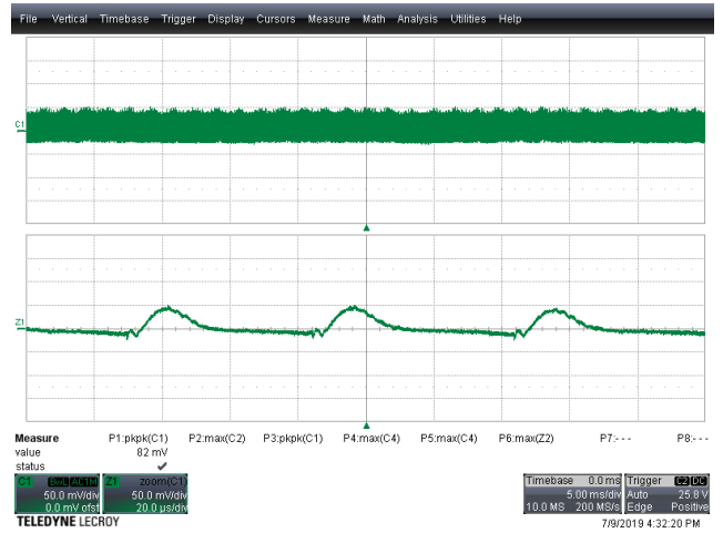
Figure 71 – Output Voltage Ripple. V_{IN} = 400 VDC, I_{OUT} = 2.5 A. Top Half: V_{OUT} , 50 mV, 5 ms / div. Bottom Half: Zoom @ 20 \mu s / div. V_{RIPPLE} = 82 mV p-p
