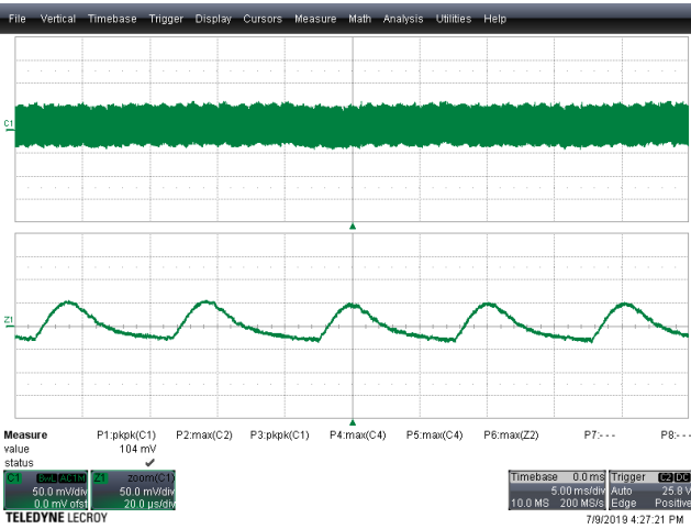
Figure 70 – Output Voltage Ripple. V_{IN} = 130 VDC, I_{OUT} = 2.5 A. Top Half: V_{OUT} , 50 mV, 5 ms / div. Bottom Half: Zoom @ 20 \mu s / div. V_{RIPPLE} = 104 mV p-p
