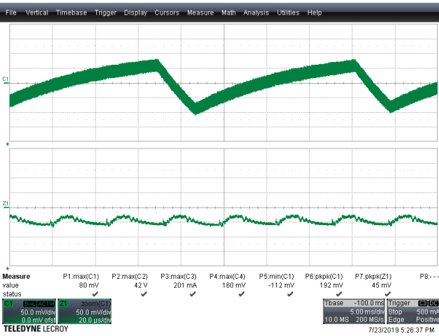
Figure 68 – Output Voltage Ripple. V_{IN} = 30 VDC, I_{OUT} = 0.85 A. Top Half: V_{OUT} , 50 mV, 5 ms / div. Bottom Half: Zoom @ 20 \mu s / div. V_{RIPPLE} = 192 mV p-p
