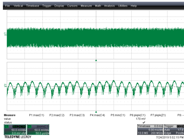
Figure 80 – Output Voltage Ripple. V_{IN} = 550 VDC, I_{OUT} = 2.5 A. Top Half: V_{OUT} , 50 mV, 5 ms / div. Bottom Half: Zoom @ 50 \mu s / div. V_{RIPPLE} = 170 mV P-P
