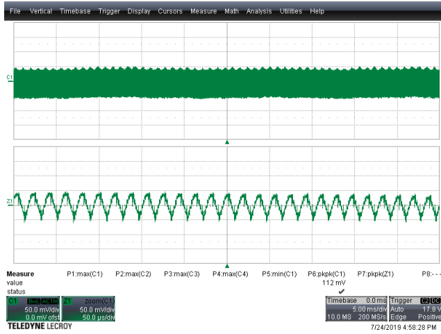
Figure 78 – Output Voltage Ripple. V_{IN} = 130 VDC, I_{OUT} = 2.5 A. Top Half: V_{OUT} , 50 mV, 5 ms / div. Bottom Half: Zoom @ 50 \mu s / div. V_{RIPPLE} = 112 mV P-P
