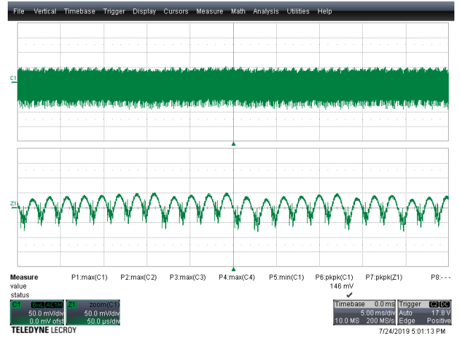
Figure 79 – Output Voltage Ripple. V_{IN} = 400 VDC, I_{OUT} = 2.5 A. Top Half: V_{OUT} , 50 mV, 5 ms / div. Bottom Half: Zoom @ 50 \mu s / div. V_{RIPPLE} = 146 mV P-P
