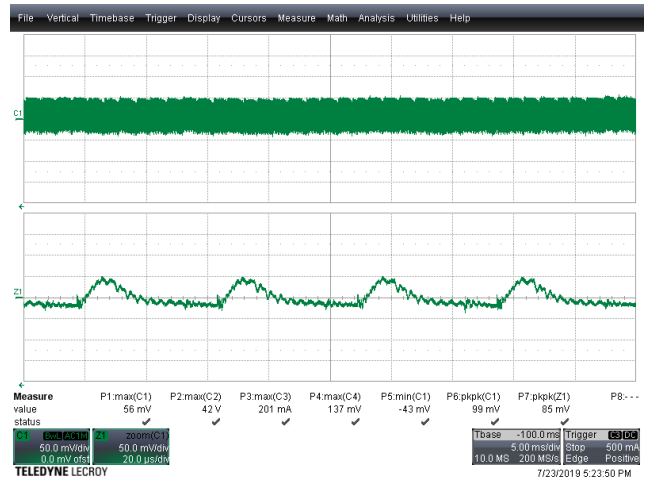
Figure 69 – Output Voltage Ripple. V_{IN} = 60 VDC, I_{OUT} = 1.25 A. Top Half: V_{OUT} , 50 mV, 5 ms / div. Bottom Half: Zoom @ 20 \mu s / div. V_{RIPPLE} = 99 mV p-p
