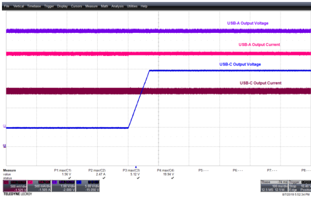
Figure 89 – 90 VAC 60 Hz, 5 – 20 V USB-C Step
