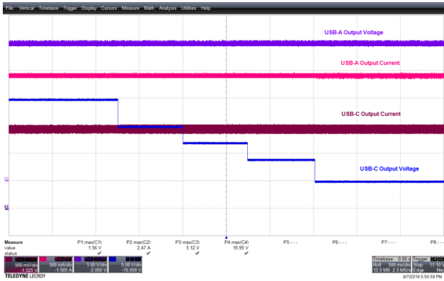
Figure 87 – 90 VAC 60 Hz, 20 V - 15 V - 12 V - 9 V - 5 V.
