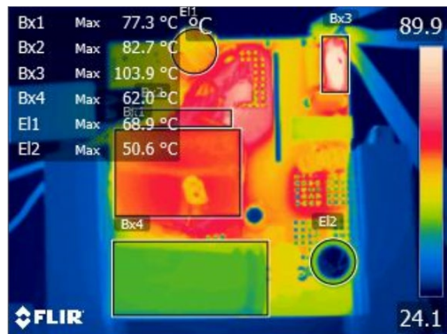
Figure 30 – Top Thermal Image, T_{AMB} = 27.9\text{ }^{\circ}\text{C} .
