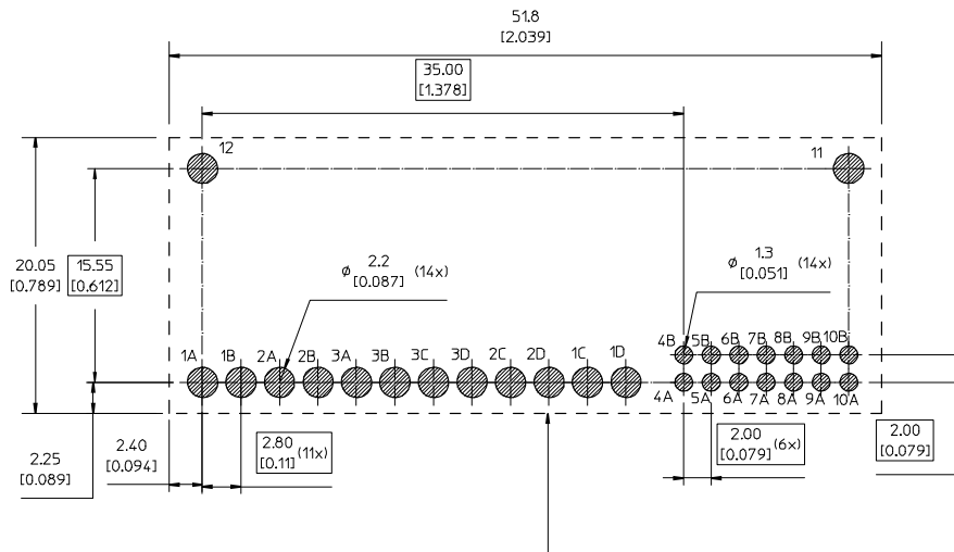
RECOMMENDED KEEP OUT AREA FOR USER COMPONENTS
