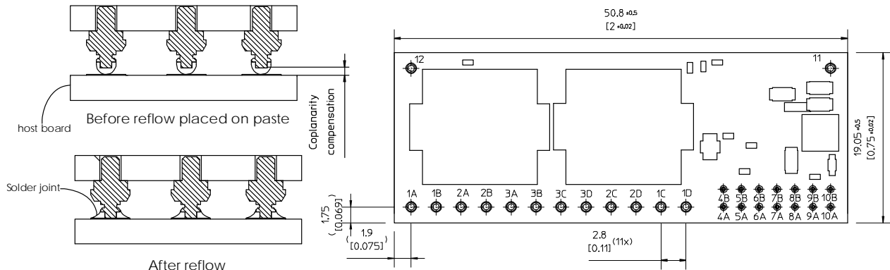
RECOMMENDED FOOTPRINT - TOP VIEW
