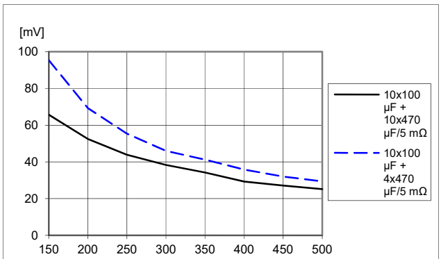
Load transient peak voltage deviation vs. ASCR gain and external capacitance. Step (22.5–67.5–22.5 A). V_i = 12\text{ V} , V_o = 1.0\text{ V} , f_{sw} = 320\text{ kHz} , ASCR residual =90, di/dt = 2\text{ A}/\mu\text{s} . ASCR gain changed by PMBus command ASCR_CONFIG.
