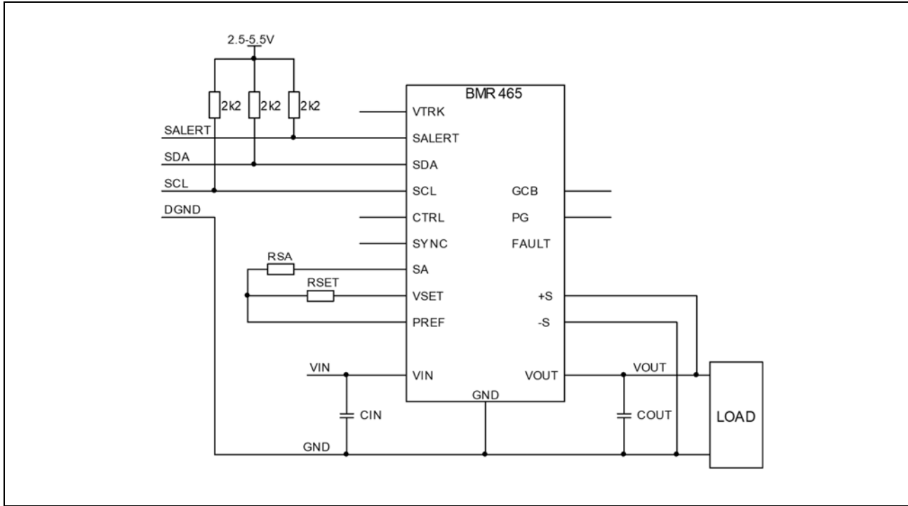
Standalone operation with PMBus communication.
