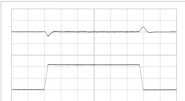
Output voltage response to load current step change (22.5–67.5–22.5 A) at V_i = 12\text{ V} , C_{OUT} = 10 \times 470\ \mu\text{F}/5\ \text{m}\Omega + 10 \times 100\ \mu\text{F} , di/dt = 2\ \text{A}/\mu\text{s} , ASCR Gain = 550 and ASCR Residual = 90. Scale from top: 50 mV/div, 20 A/div, 100 \mu\text{s}/\text{div} .
