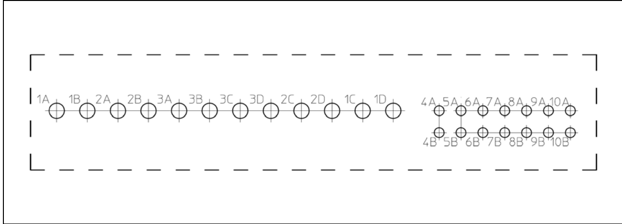
Pin layout, top view.
