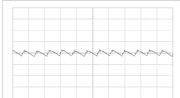
Fundamental output voltage ripple at V_i = 12\text{ V} , I_o = \text{max } I_o , C_{OUT} = 10 \times 470\ \mu\text{F}/5\ \text{m}\Omega + 10 \times 100\ \mu\text{F} . Scale: 5 mV/div, 2 \mu\text{s}/\text{div} , 20 MHz bandwidth. See section Output Ripple and Noise.
