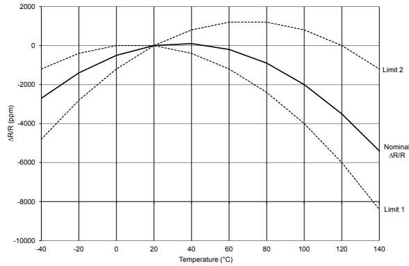
FIGURE 1 – TEMPERATURE COEFFICIENT
