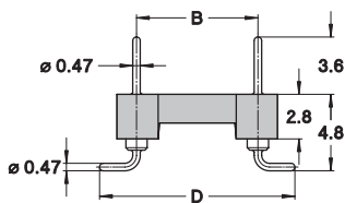
INSULATOR
