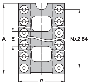
INSULATOR
