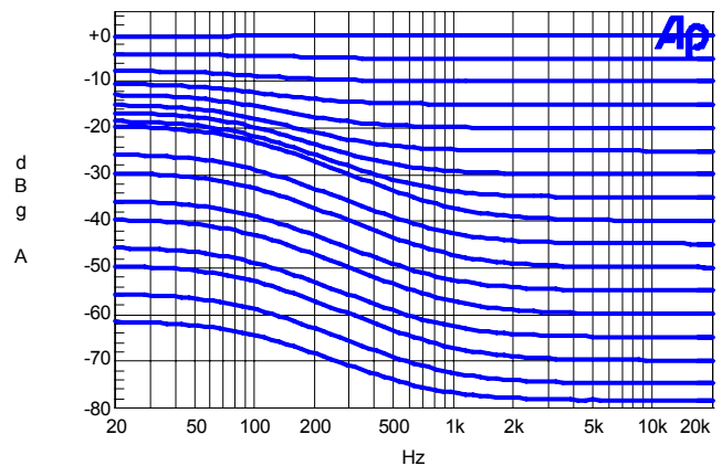
PT7314E Loudness Response VS Master Volume
