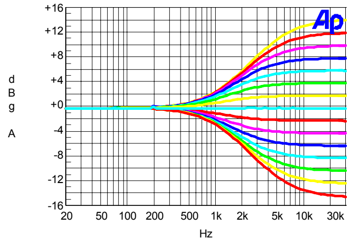
Treble Response
