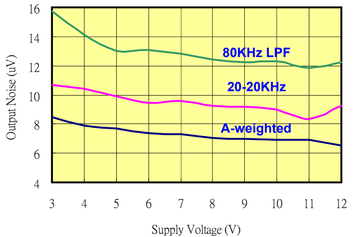
Residual Noise
