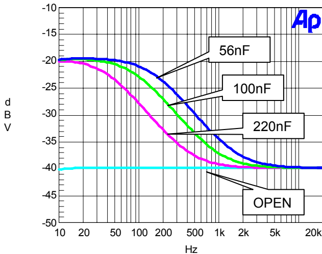
PT7314E Loudness Response VS CAP (Volume=-40dB)
