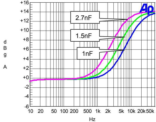
PT7314E Treble Response VS CAP
