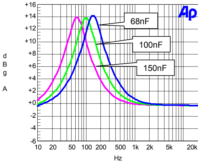
PT7314E Bass Response VS CAP
