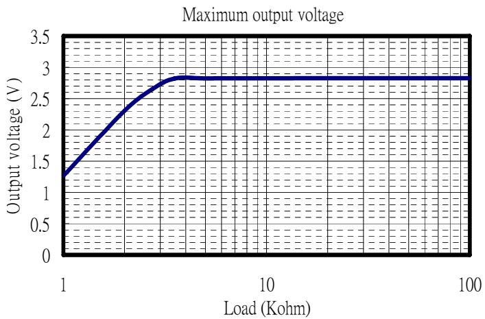
Maximum Output Level VS R LOAD
