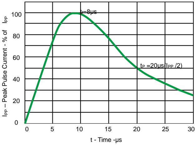
Fig 1. Pulse Waveform
