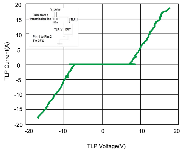
Fig 6. TLP Measurement
