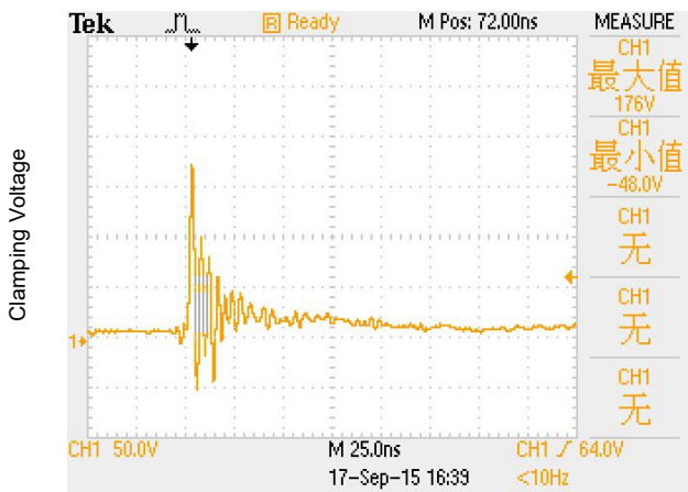
ESD clamping
