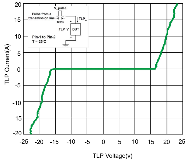
Fig 6. TLP Measurement
