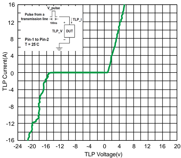
Fig 5. TLP Measurement
