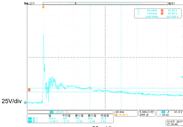
20ns/div Fig 7. ESD clamping voltage (IEC61000-4-2 +8KV contact)
