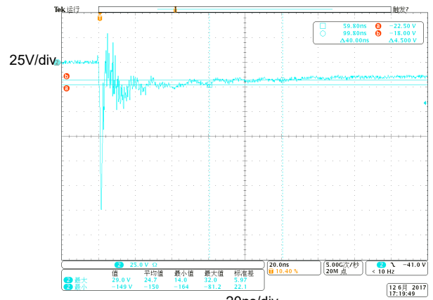
20ns/div Fig 8. ESD clamping voltage (IEC61000-4-2 -8KV contact)
