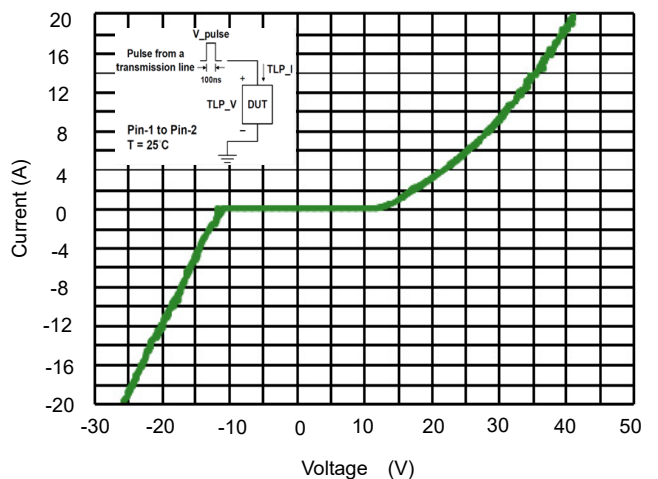
Fig 6. TLP Measurement
