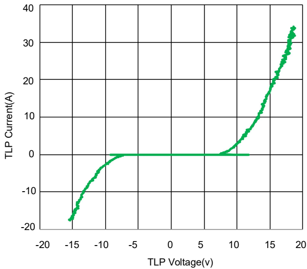
Fig 5. TLP Measurement
