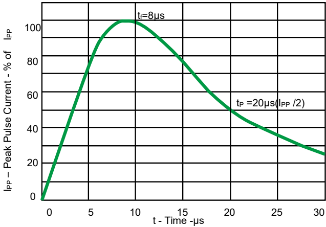
Fig 1. Pulse Waveform
