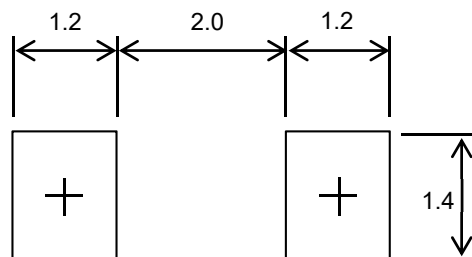
Suggested PCB Layout Unit:mm
