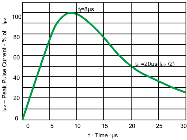
Fig 1. Pulse Waveform
