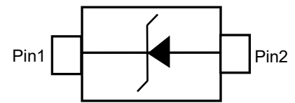
Circuit Diagram
