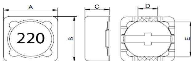
PSPHAQ73/74124/125/127/129尺寸图
