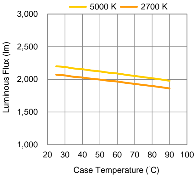
Fig 4. Case Temperature vs. Luminous Flux at 500 mA.
