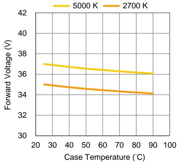
Fig 5. Case Temperature vs. Forward Voltage at 500 mA.
