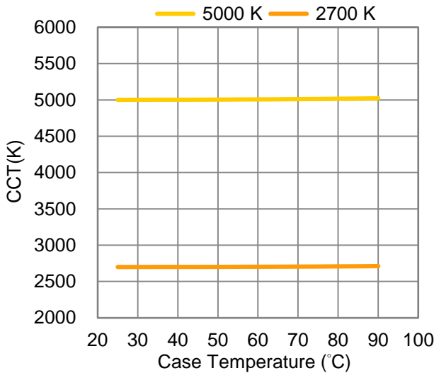
Fig 6. Case Temperature vs. Chromaticity Coordinate \Delta x at 500 mA.
