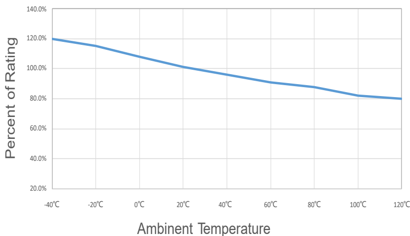
Temperature Re-rating Curve
