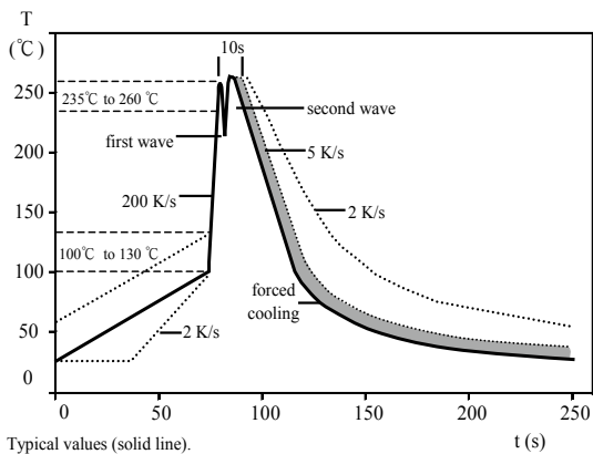
WAVE soldering.
