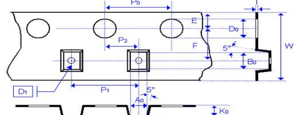
Fig. 9.2 The dimension of plastic tape
