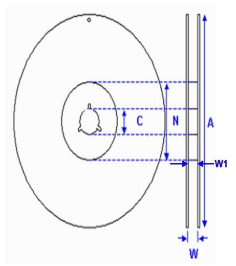
Fig. 9.3 The dimension of reel
