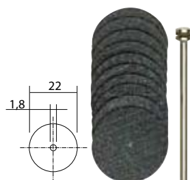
NO 28 808 10 pieces Aluminium oxide cutting discs with reinforcement The cutting discs are available in \varnothing 22 x 0.8 and \varnothing 38 x 1. Nearly unbreakable, making them usable to remove stock. Will cut alloyed, standard and stainless steels, non-ferrous metals and even wood and plastic. Arbor shaft of \varnothing 2.35.
