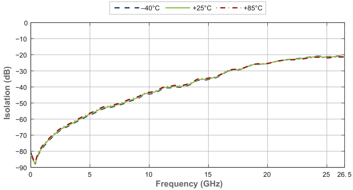
Figure 14 • Isolation vs Temperature (RFX–RFX)
