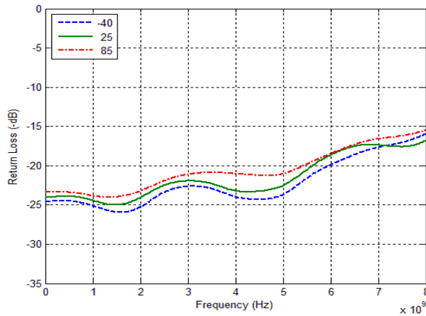
Figure 10. Active Port Return Loss vs. Temp
