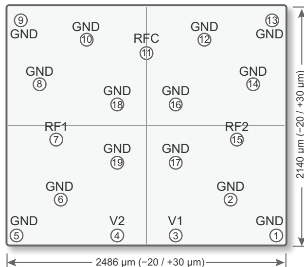
Figure 15 • Pin Layout for PE42524 (1)(2)
