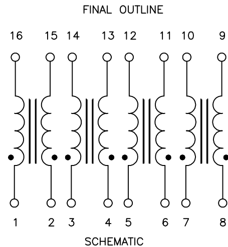
SCHEMATIC
