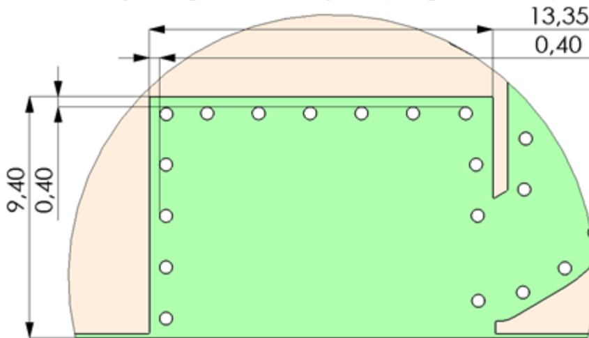
DETAIL C
