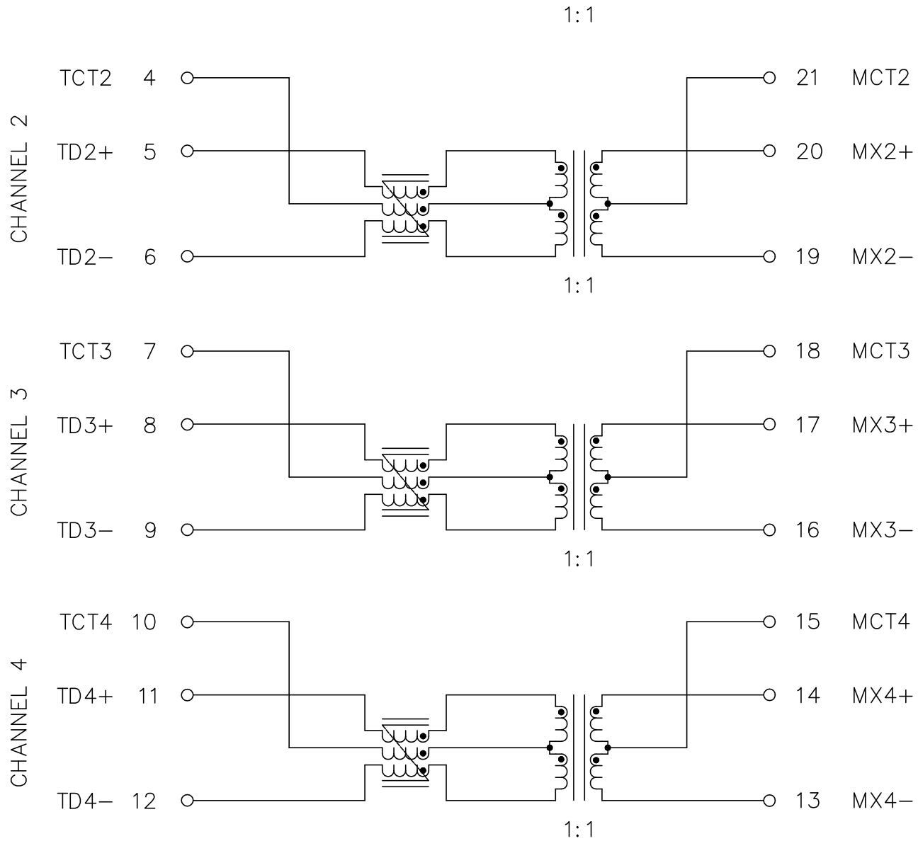
SCHMATIC
