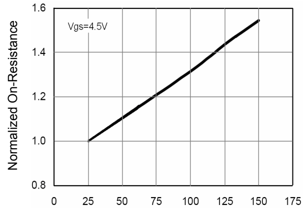
Tj-Junction Temperature( ^\circ\text{C} ) Figure 8 Drain-Source On-Resistance
