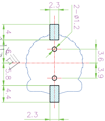
POB Holes Diagram Top View
