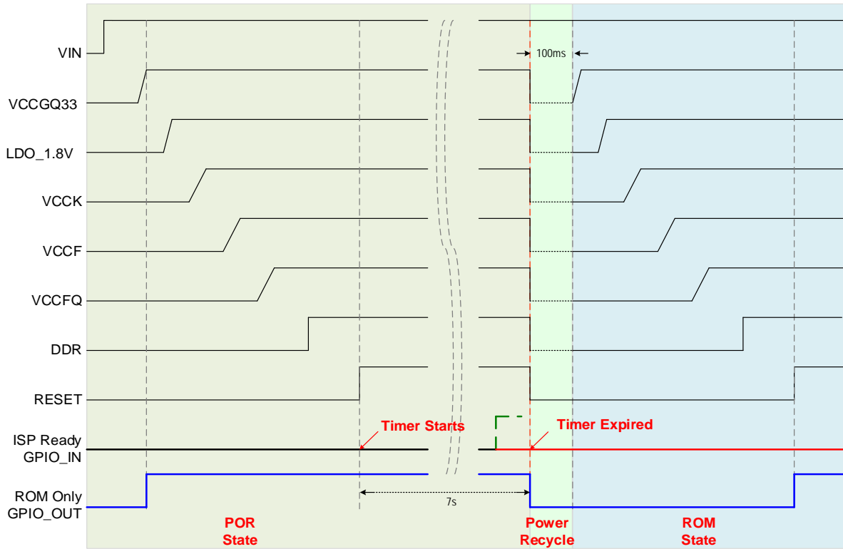
Figure 6: ROM State
