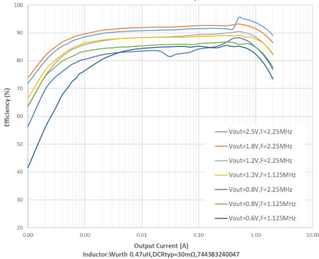
Buck5 Efficiency, VIN = 3.3V
