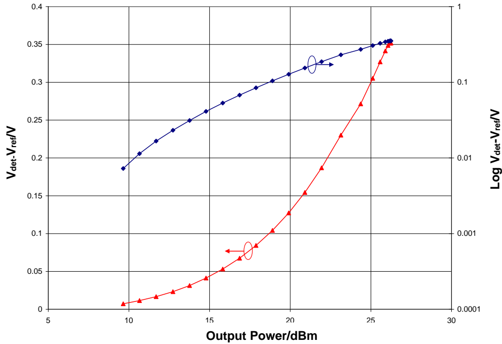
Detector Voltage ( V_{ref}-V_{det} ), V_{dd} = 5.0\text{ V} , I_{dd} = 480\text{ mA} , F = 30\text{ GHz}
