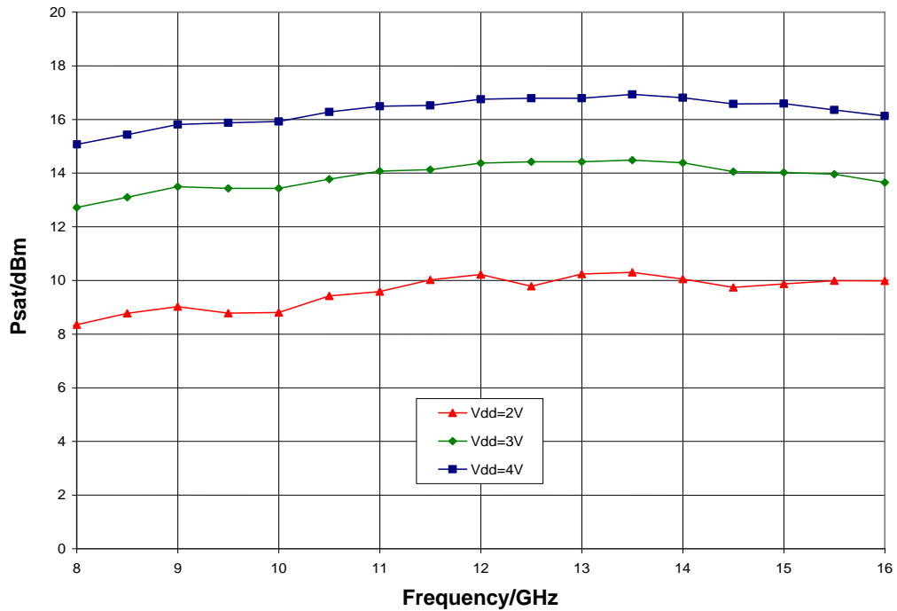
Psat vs. V_{dd} , T_A = 25^\circ\text{C}
