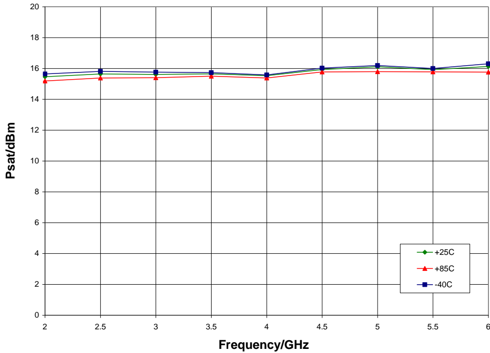
Psat vs. Temperature, V dd = 4.0 V
