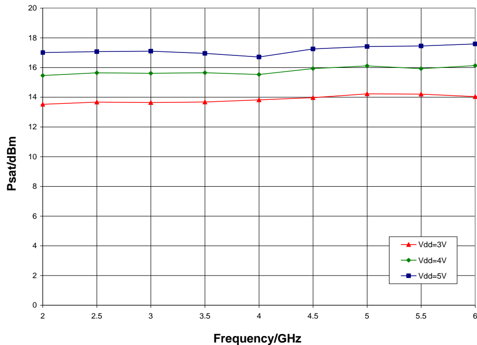
Psat vs. V dd , T A = 25° C
