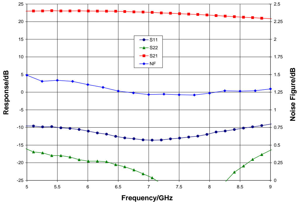
Narrow-band Performance, V_{dd} = 3.6\text{ V} , T_A = 25^\circ\text{ C}
