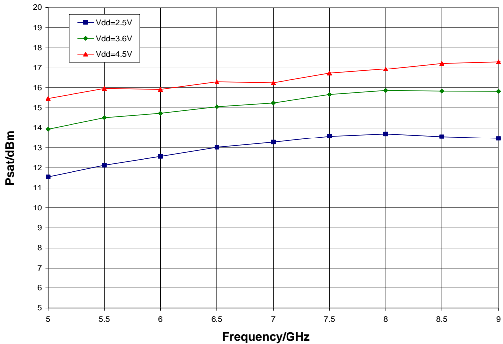
Psat vs. V dd , T A = 25° C
