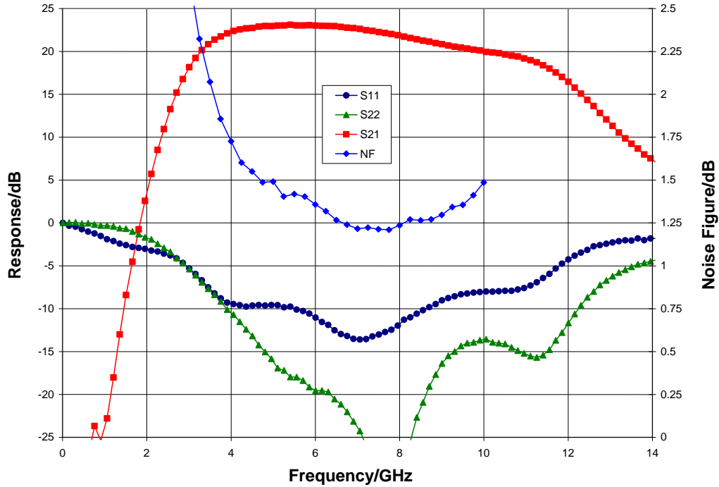
Broadband Performance, V_{dd} = 3.6\text{ V} , T_A = 25^\circ\text{ C}
