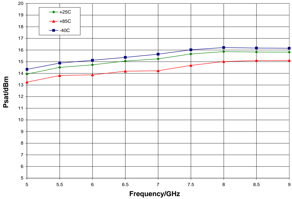
Psat vs. Temperature, V dd = 3.6 V
