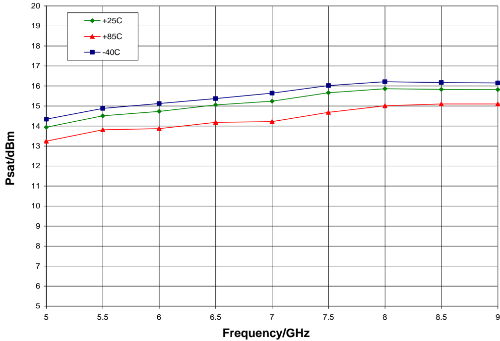
Psat vs. Temperature, V dd = 3.6 V
