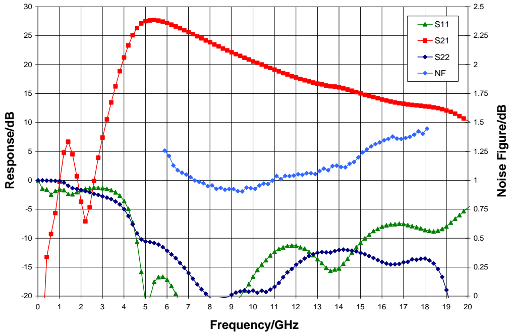
Broadband Performance, V_{dd} = 3\text{ V} , V_{gg} = 1.5\text{ V} , T_A = 25^\circ\text{C}
