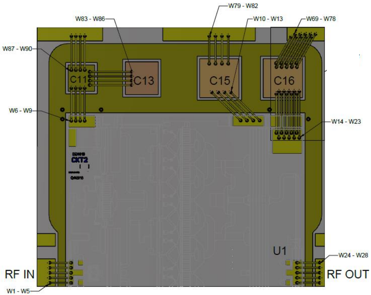
DETAIL C
