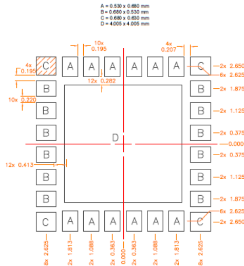
PCB Solder Mask Pattern
