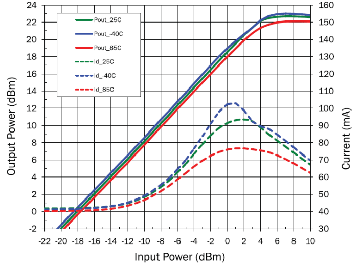
Output Power versus Input Power ( V_D = 5\text{V} )
