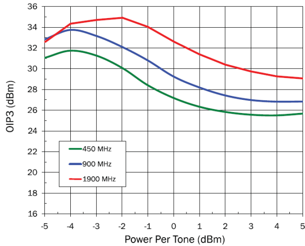
OIP3 versus Power Out ( V_D = 5\text{V} , 25C)
