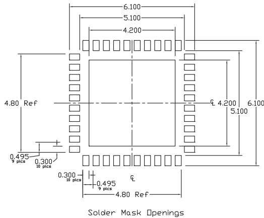
Solder Mask Openings
