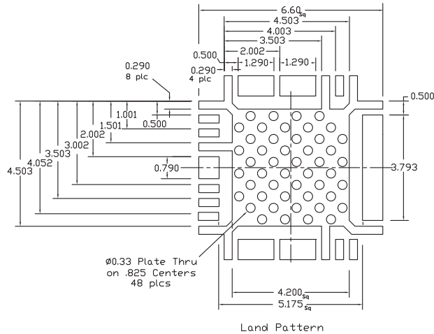
Land Pattern
