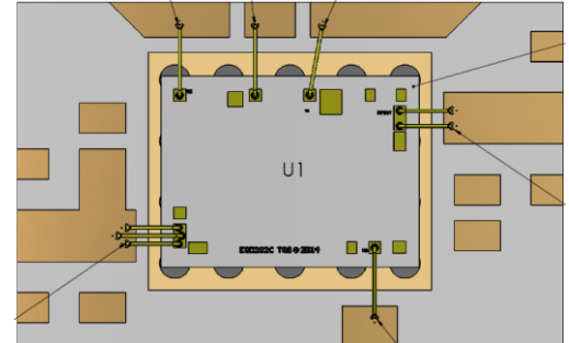
MMIC mounting/wire bonding detail
