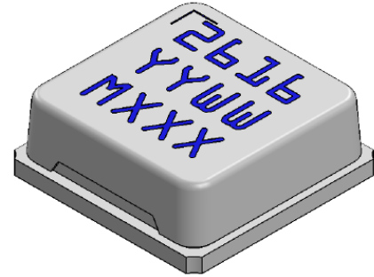
4 x 4 mm Air Cavity QFN Package
